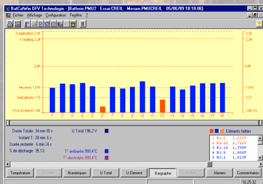
Voltage of each cell
